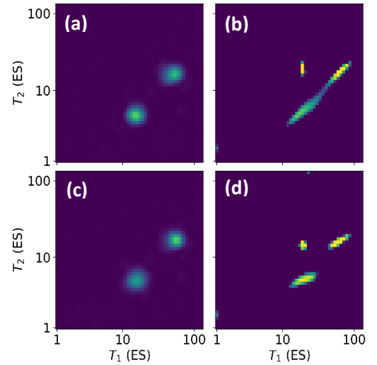
Figure 2. The T_1 - T_2 spectra, with two peaks at ( T_1 64ES, T_2 20ES) and ( T_1 16ES, T_2 5ES), produced by NN (1 st column) and ILT (2 nd column, regularization 0.01). There was no noise in (a) and (b) signals. (c) and (d) had 200 SNR. The true spectrum is shown in Fig. 1b.
