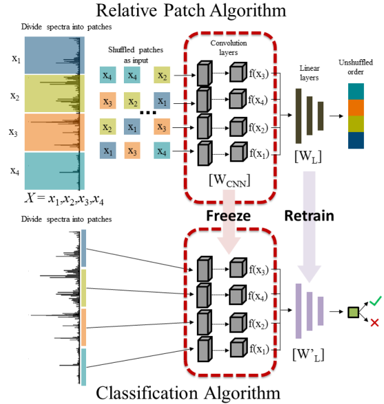
Fig 1: Overview of the network architecture and workflow
